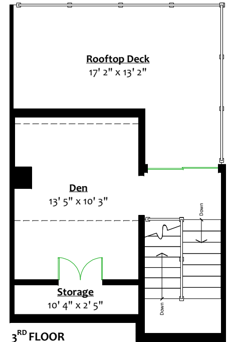
3 RD FLOOR Floor Area: 292 Sq. Ft. Ceiling Height: 7'
