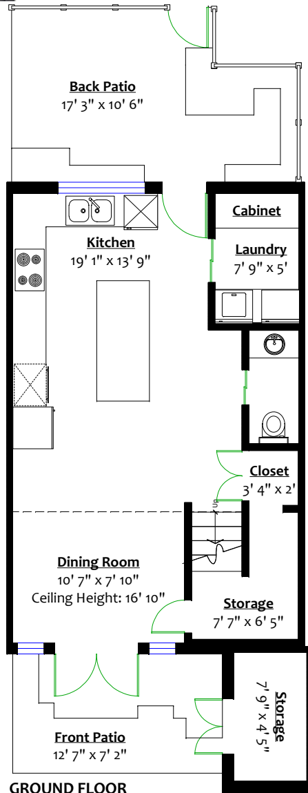
GROUND FLOOR Floor Area: 503 Sq. Ft. Ceiling Height: 7' 7"
