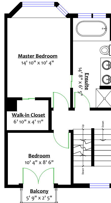
2 ND FLOOR Floor Area: 505 Sq. Ft. Ceiling Height: 8'
